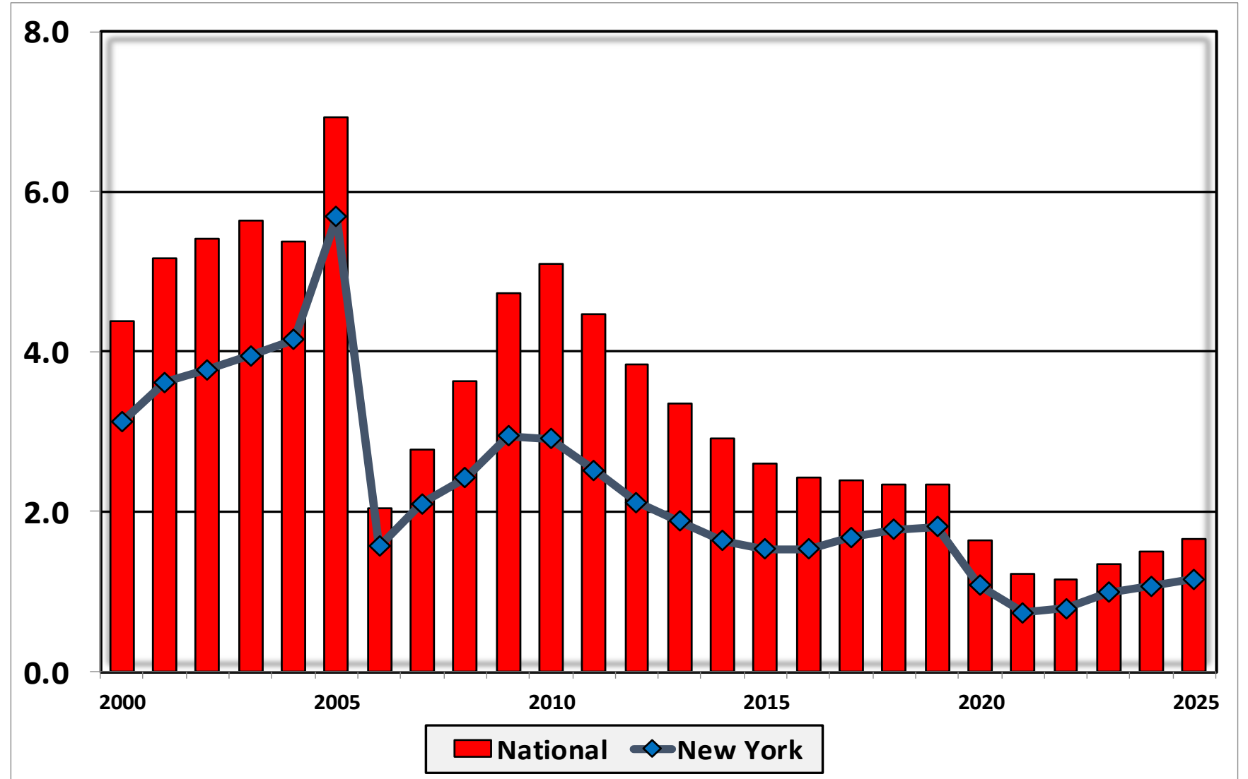
Bankruptcy Filings per 1,000 Population New York vs. National Average 2000 - 2025
