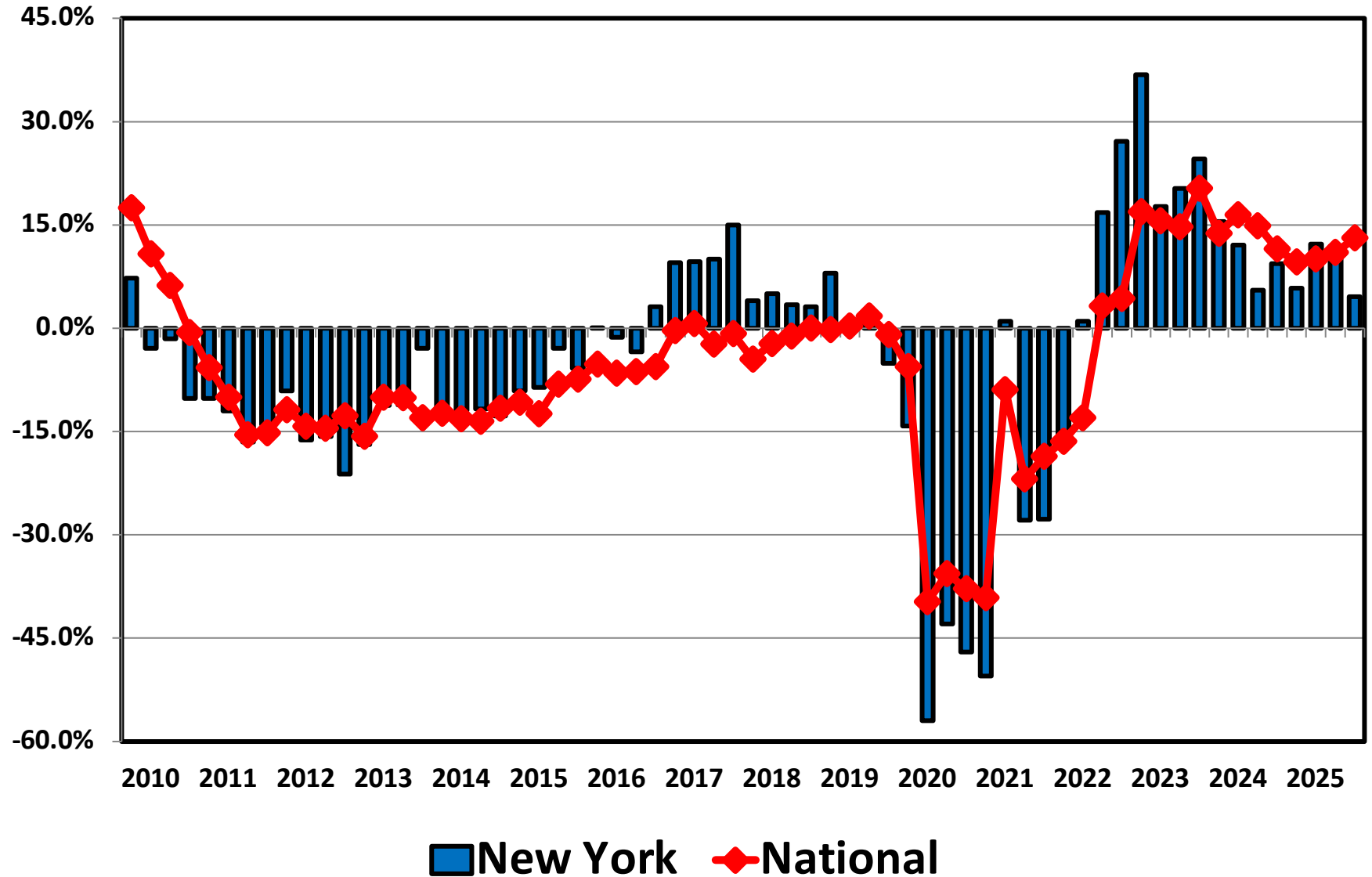
Filing Trends By Quarter New York vs. National Average (Percent Change From Same Quarter One Year Prior)
